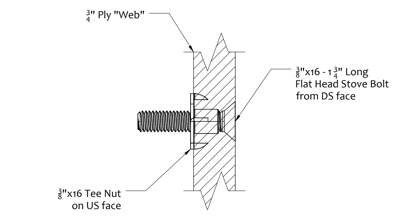
2 159 Angle Iron Bolt Detail Side View 1'-0" = 1'-0" Affix stove bolts through "web" plywood Before covering DS face with 20ga Steel
