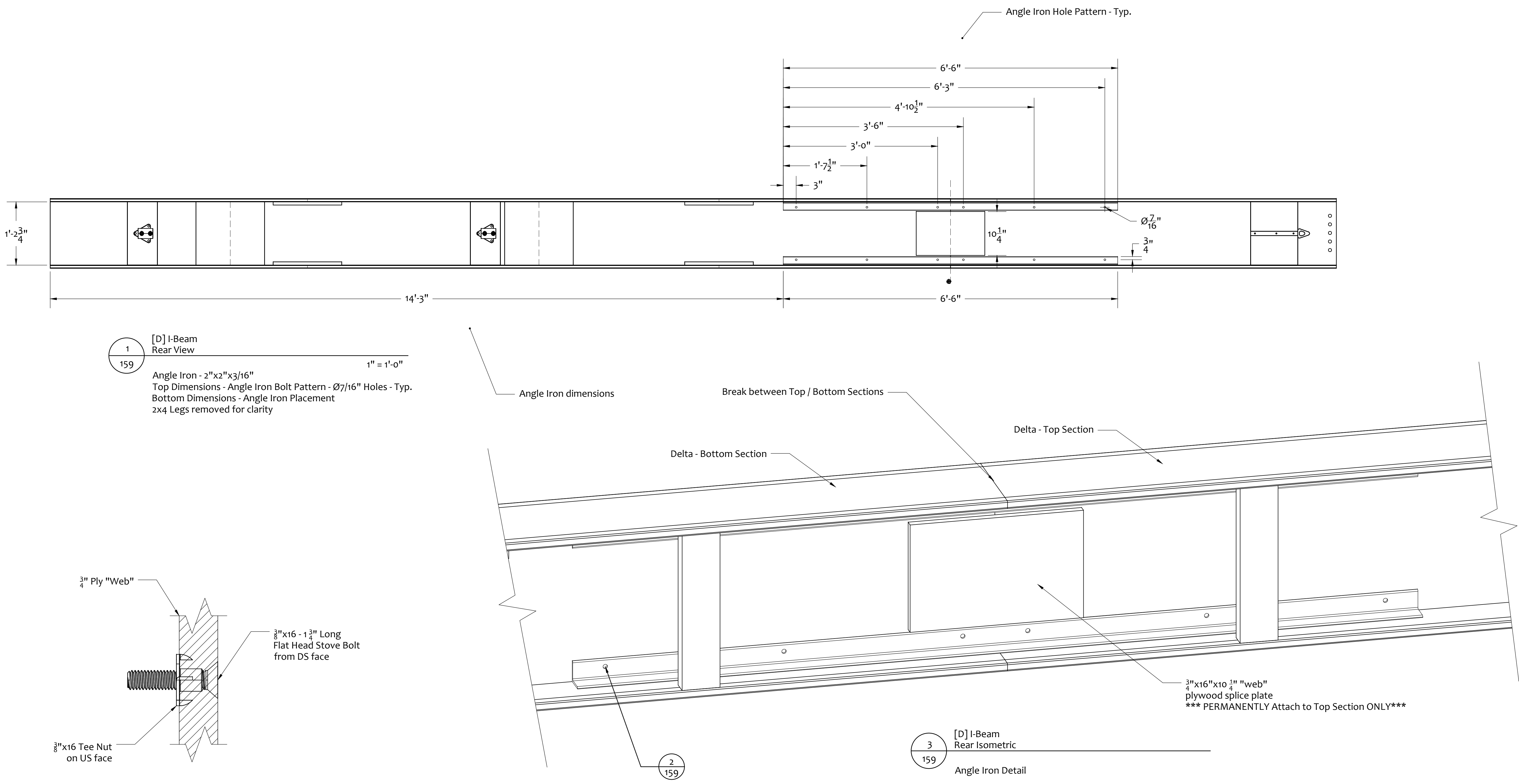
2 159 Angle Iron Bolt Detail Side View 1'-0" = 1'-0" Affix stove bolts through "web" plywood Before covering DS face with 20ga Steel
